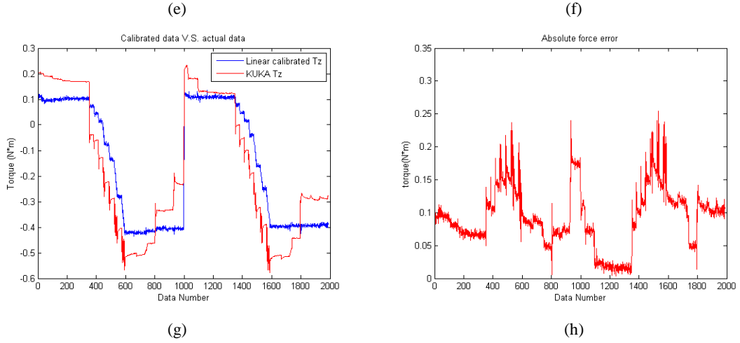
Figure 5.14: Linear calibrated (two parameters)force and torque from sensor versus actual data from robotic arm (a) evaluation of normal force F_z ; (b) absolute error performance of F_z under two set of normal force from 0 N to -40N(compression); (c) evaluation of normal force F_x ; (d) absolute error performance of F_x under one set of shear force from 0 N to -15N; (e) evaluation of normal force F_y ; (f) absolute error performance of F_y under one set of shear force from 0 N to -15N; (g) evaluation of normal force T_z ; (h) absolute error performance of T_z under two set of Torque from 0 N·m to 0.8 N·m.
