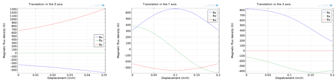
Figure 4.7: Simulation of magnetic flux density for three axes while translating across a rectangular magnet with length over width ratio of 1/2 in the Z, Y, and X axes.
