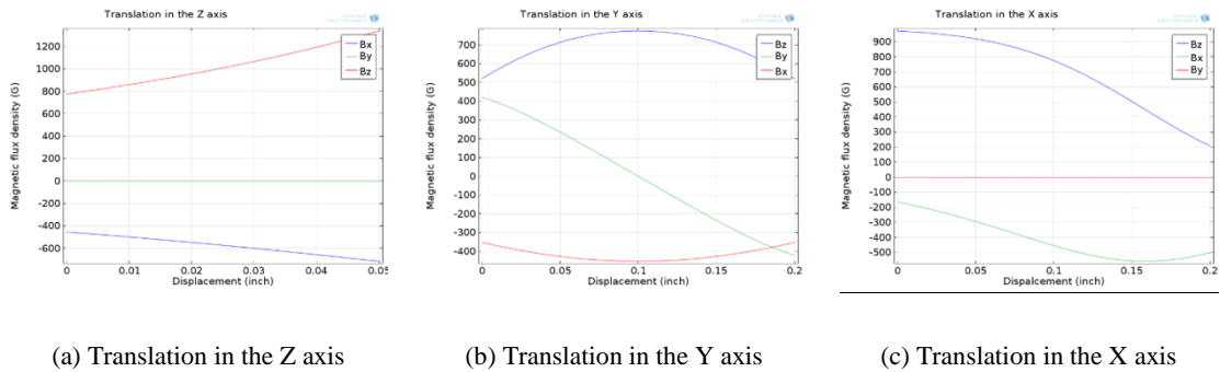
Figure 4.7: Simulation of magnetic flux density for three axes while translating across a rectangular magnet with length over width ratio of 1/2 in the Z, Y, and X axes.
