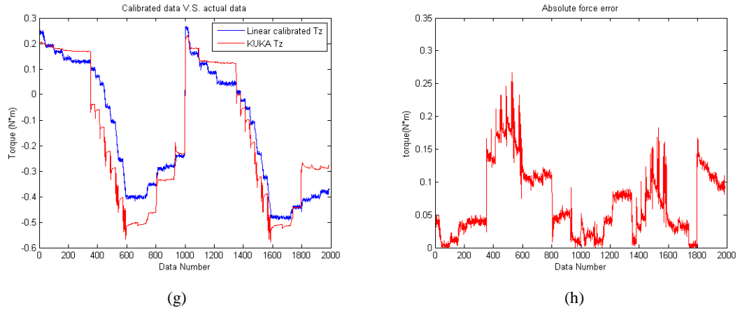
Figure 5.15: Linear calibrated (five parameters)force and torque from sensor versus actual data from robotic arm (a) evaluation of normal force F_z ; (b) absolute error performance of F_z under two set of normal force from 0 N to -40N(compression); (c) evaluation of normal force F_x ; (d) absolute error performance of F_x under one set of shear force from 0 N to -15N; (e) evaluation of normal force F_y ; (f) absolute error performance of F_y under one set of shear force from 0 N to -15N; (g) evaluation of normal force T_z ; (h) absolute error performance of T_z under two set of Torque from 0 N·m to 0.8 N·m.
